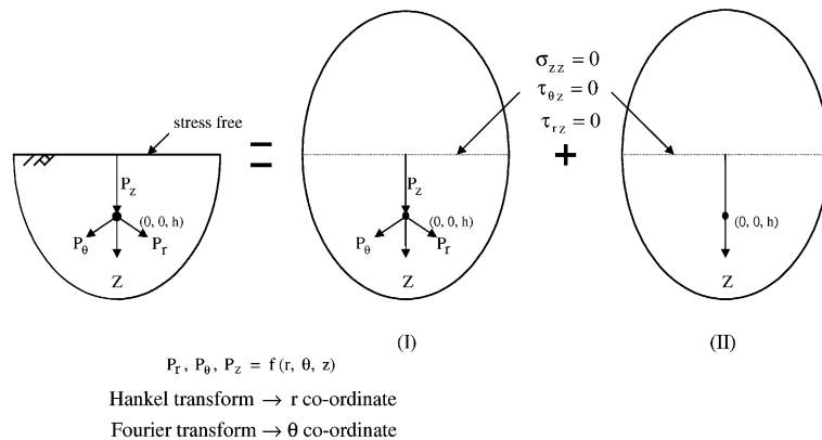
Fig. 1. The approach for solving a point load problem (Liao and Wang, 1998).
